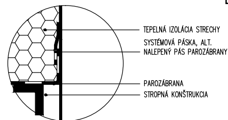
DETAIL I
