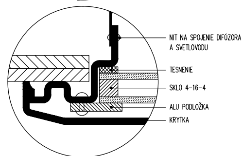
DETAIL II
